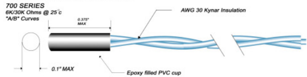
LS700 Series 6k Ohms at 25°C A Curve 30k Ohms at 25°C B Curve
