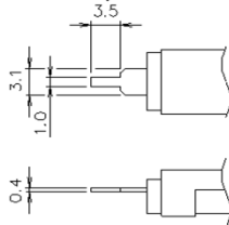
TERMINAL TYPE g
