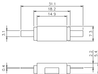
TERMINAL TYPE f
